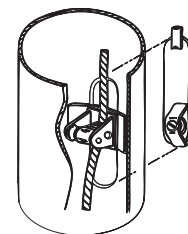
Internal Cam Cleat & Handhole Door
